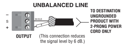
Figure 2.5 Line Out Wiring. Top: Balanced. Bottom: Unbalanced.
